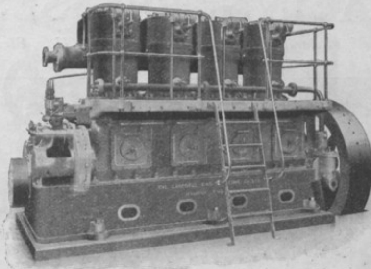
HIGH COMPRESSION OIL ENGINE, 140 B.H.P.
