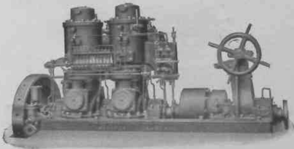
66 B.H.P. MARINE OIL ENGINE, GEAR REVERSE TYPE.
